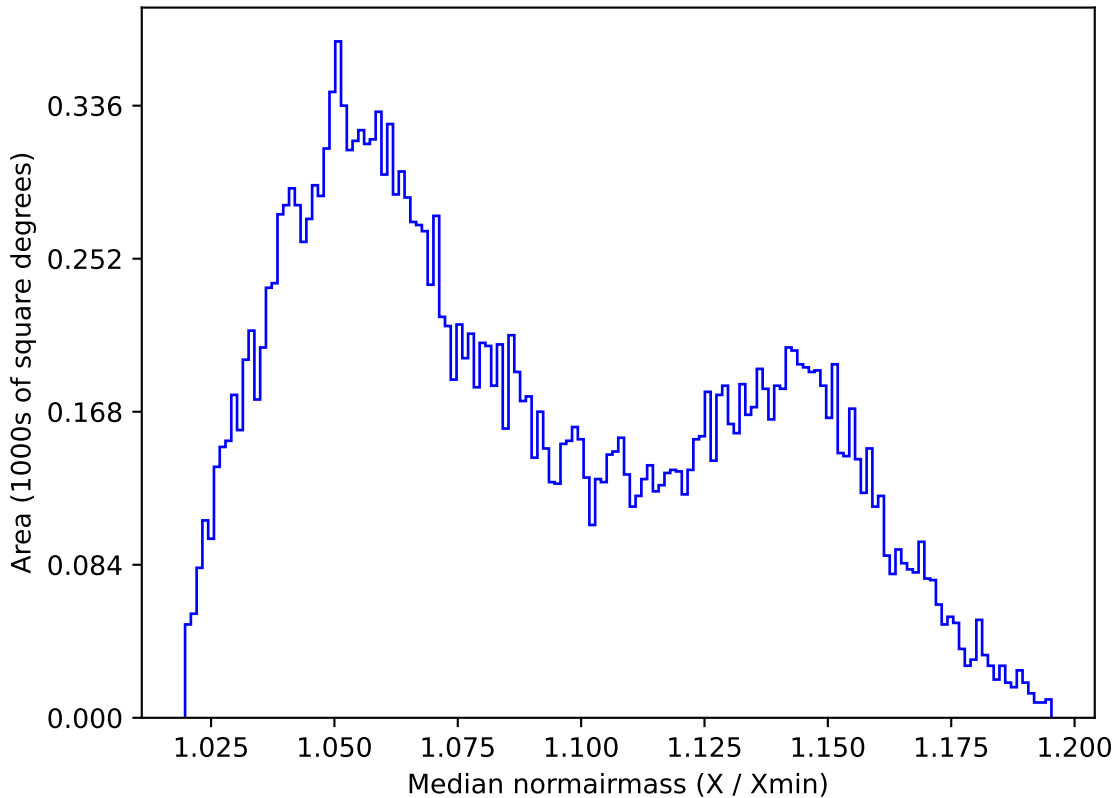
ddf_acor_sf25_lsf40_lsr20_v3.4_10yrs All sky y band: Median normairmass
