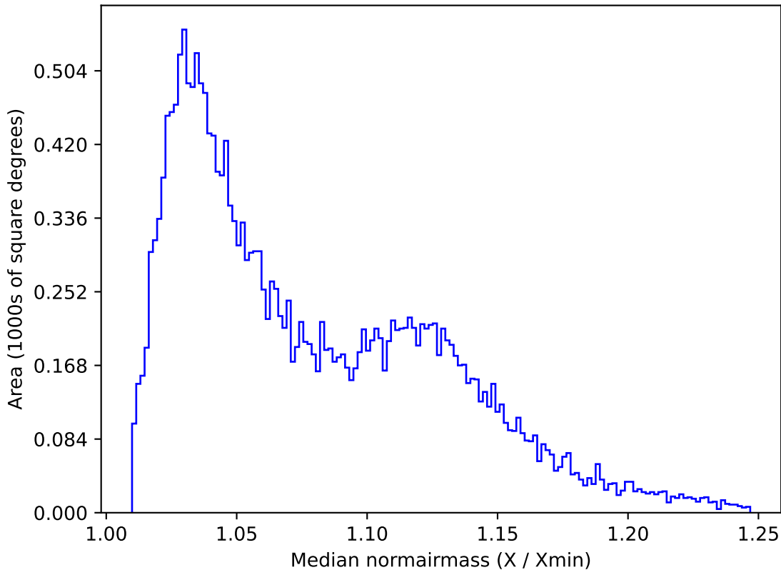
ddf_acor_sf25_lsf40_lsr20_v3.4_10yrs All sky u band: Median normairmass
