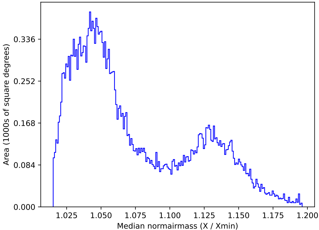
ddf_acor_sf25_lsf40_lsr20_v3.4_10yrs All sky r band: Median normairmass
