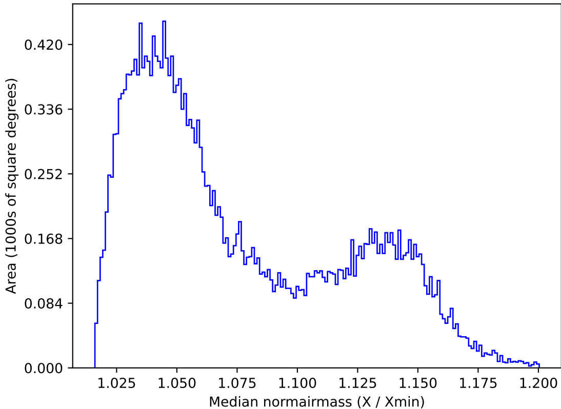
ddf_acor_sf25_lsf40_lsr20_v3.4_10yrs All sky i band: Median normairmass
