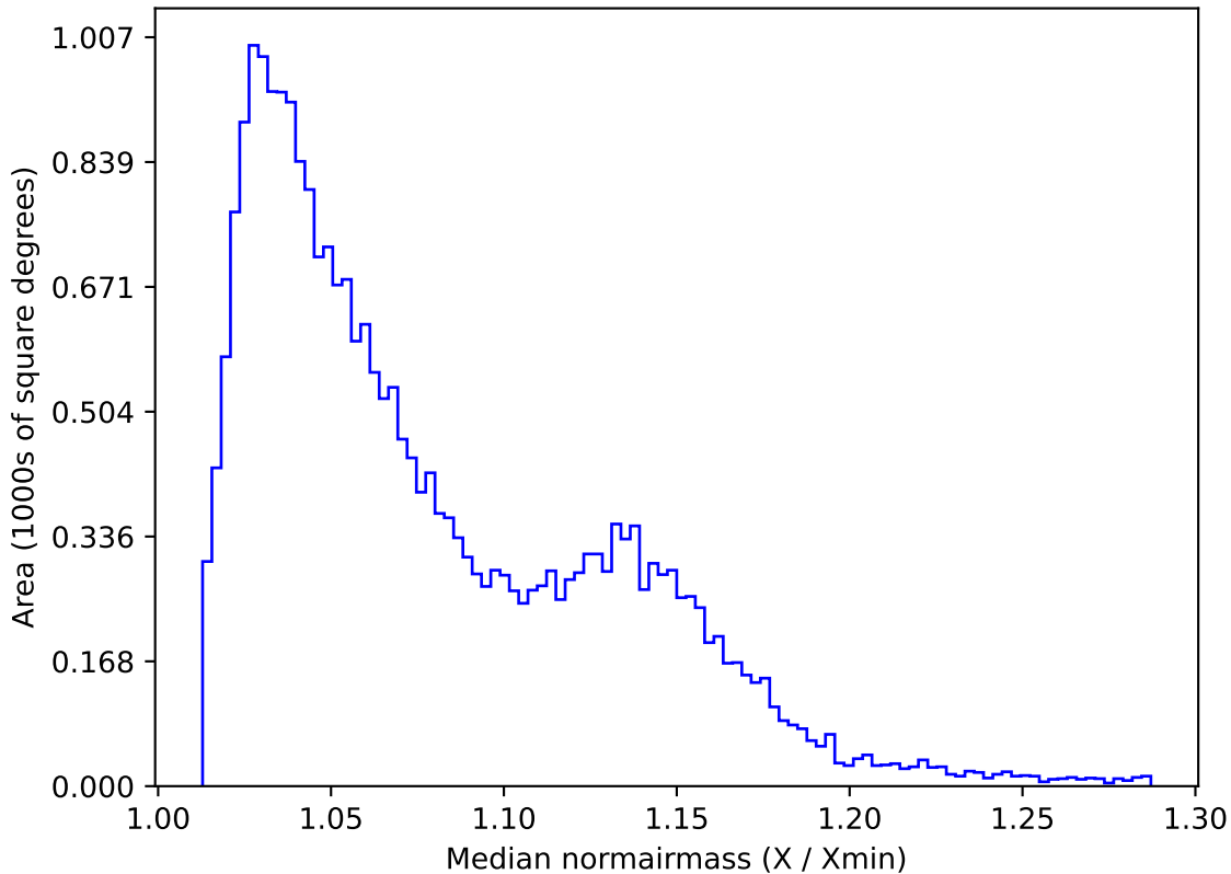
ddf_acor_sf25_lsf40_lsr20_v3.4_10yrs All sky g band: Median normairmass
