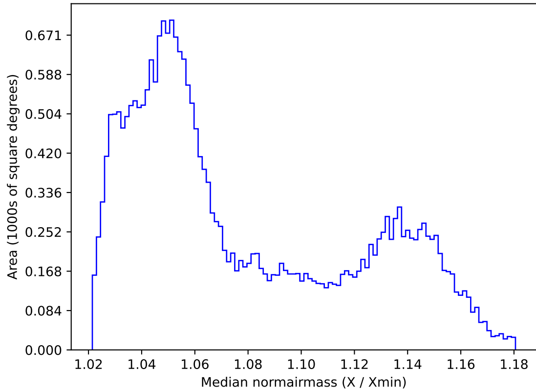
ddf_acor_sf25_lsf40_lsr20_v3.4_10yrs All sky all bands: Median normairmass
