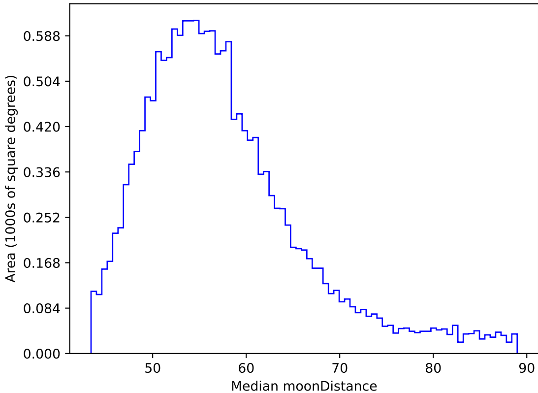
ddf_acor_sf25_lsf40_lsr20_v3.4_10yrs WFD y band: Median moonDistance
