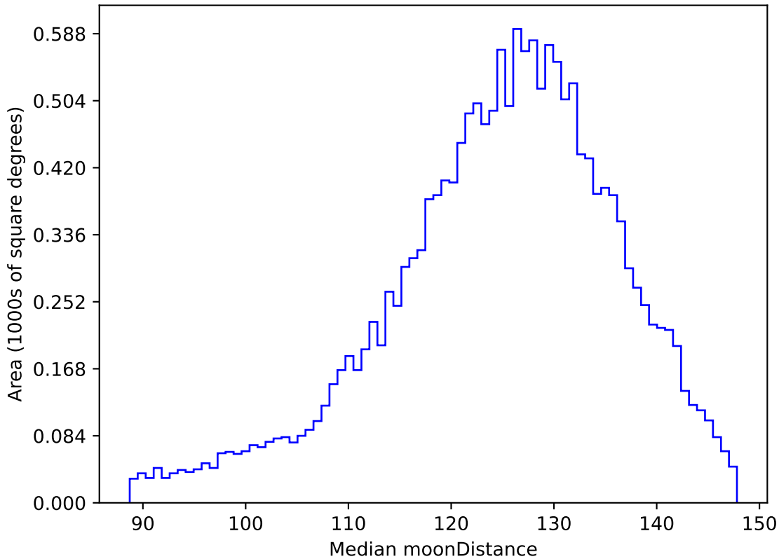
ddf_acor_sf25_lsf40_lsr20_v3.4_10yrs WFD u band: Median moonDistance
