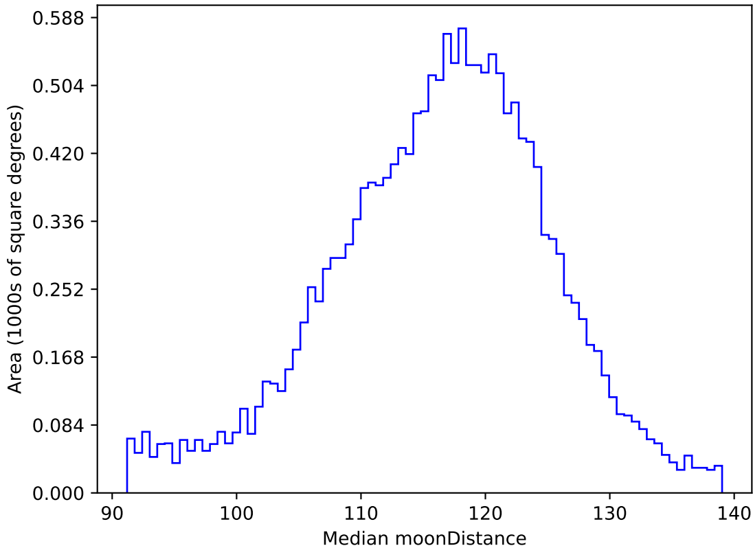
ddf_acor_sf25_lsf40_lsr20_v3.4_10yrs WFD g band: Median moonDistance
