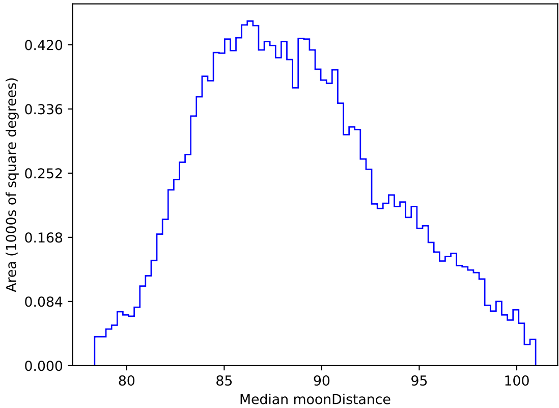
ddf_acor_sf25_lsf40_lsr20_v3.4_10yrs WFD all bands: Median moonDistance
