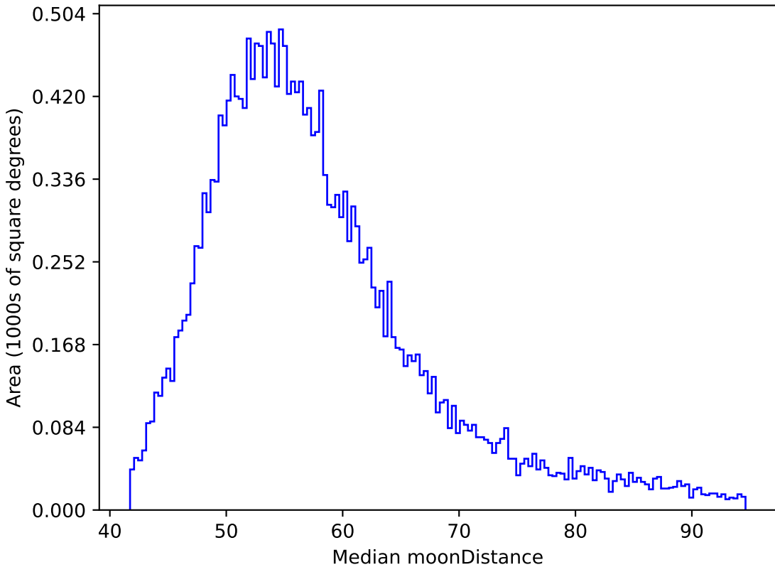
ddf_acor_sf25_lsf40_lsr20_v3.4_10yrs All sky y band: Median moonDistance
