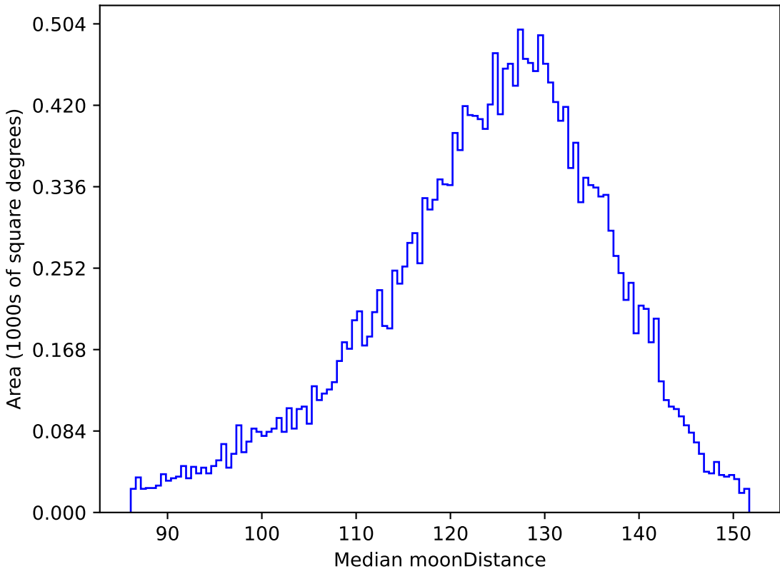
ddf_acor_sf25_lsf40_lsr20_v3.4_10yrs All sky u band: Median moonDistance
