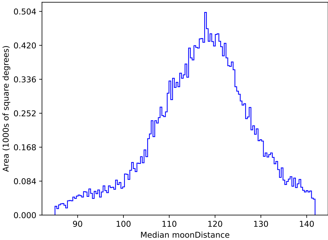
ddf_acor_sf25_lsf40_lsr20_v3.4_10yrs All sky g band: Median moonDistance
