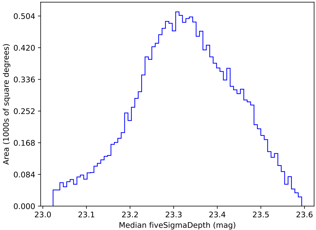
ddf_acor_sf25_lsf40_lsr20_v3.4_10yrs WFD all bands: Median fiveSigmaDepth
