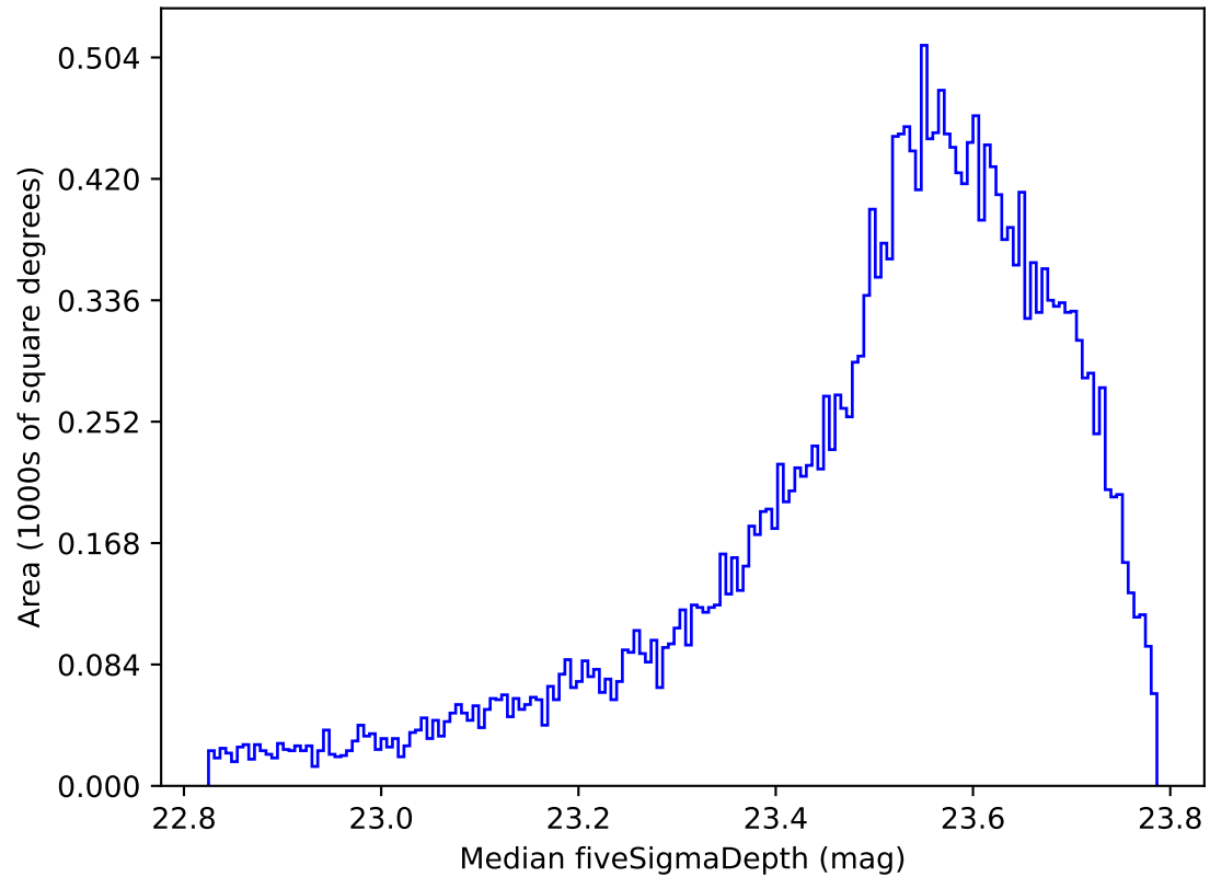
ddf_acor_sf25_lsf40_lsr20_v3.4_10yrs All sky i band: Median fiveSigmaDepth
