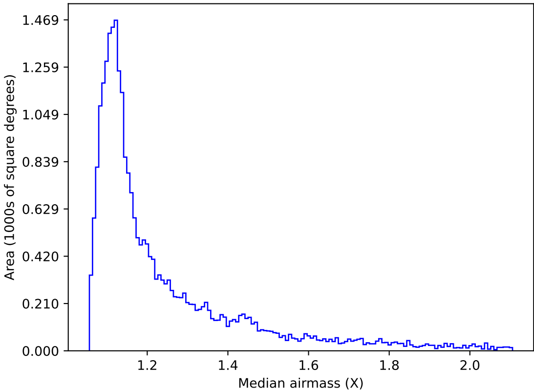
ddf_acor_sf25_lsf40_lsr20_v3.4_10yrs Yr 1 r band: Median airmass
