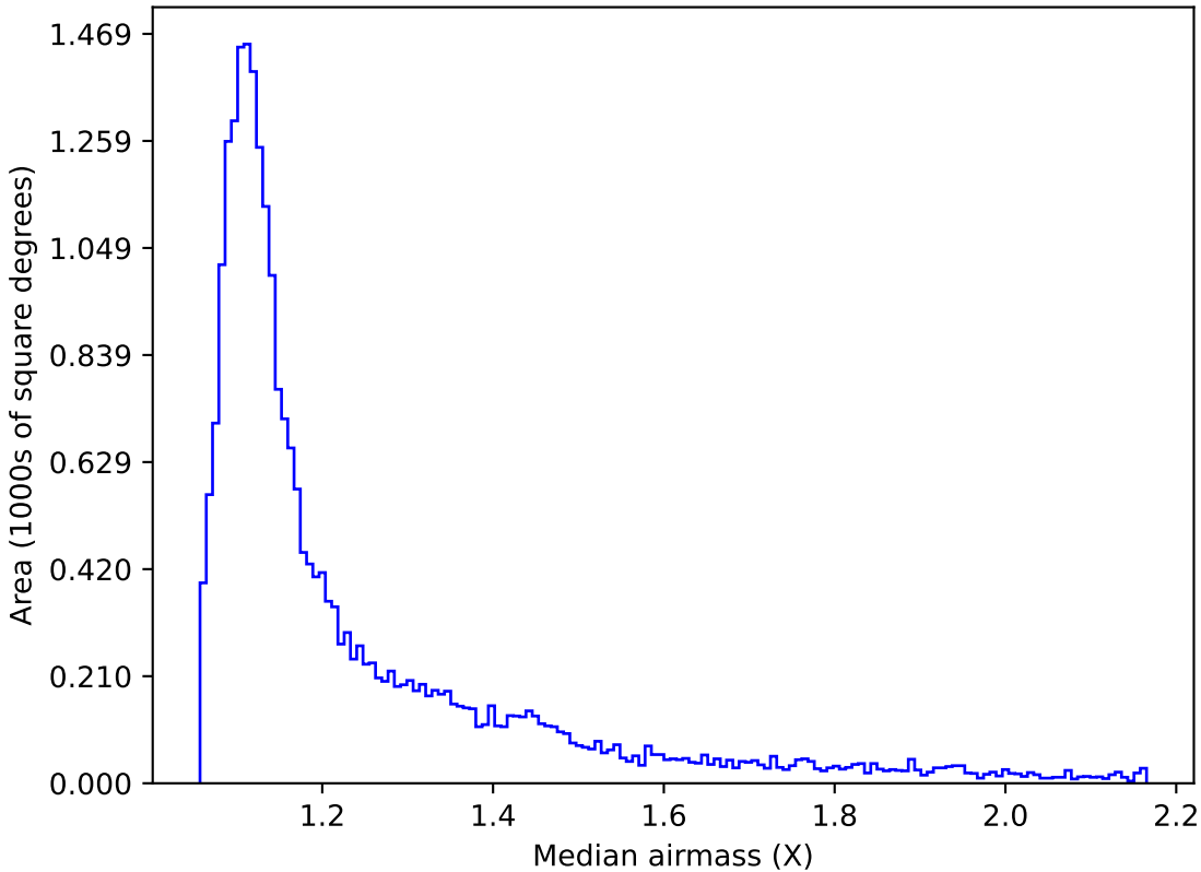
ddf_acor_sf25_lsf40_lsr20_v3.4_10yrs Yr 1 i band: Median airmass
