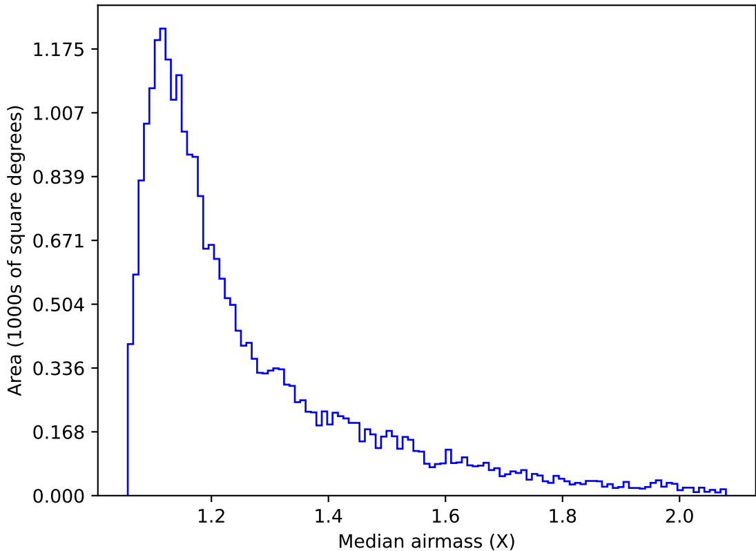
ddf_acor_sf25_lsf40_lsr20_v3.4_10yrs Yr 1 g band: Median airmass
