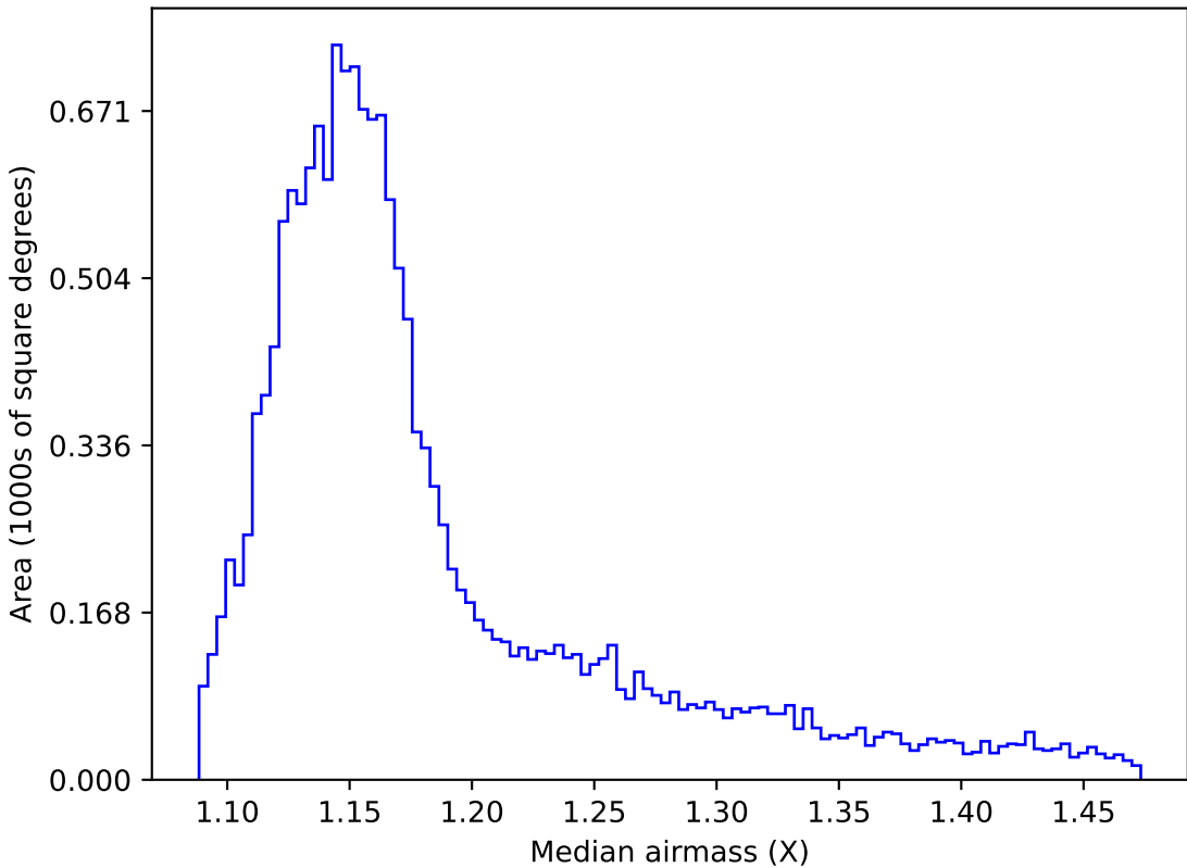
ddf_acor_sf25_lsf40_lsr20_v3.4_10yrs WFD z band: Median airmass
