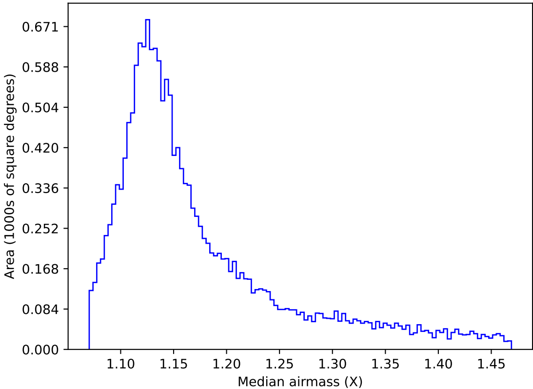
ddf_acor_sf25_ls40_lsr20_v3.4_10yrs WFD u band: Median airmass
