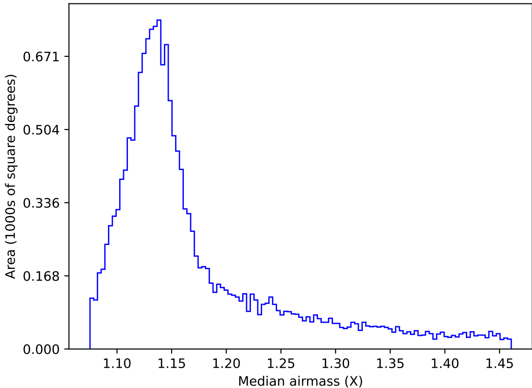
ddf_acor_sf25_lsf40_lsr20_v3.4_10yrs WFD r band: Median airmass
