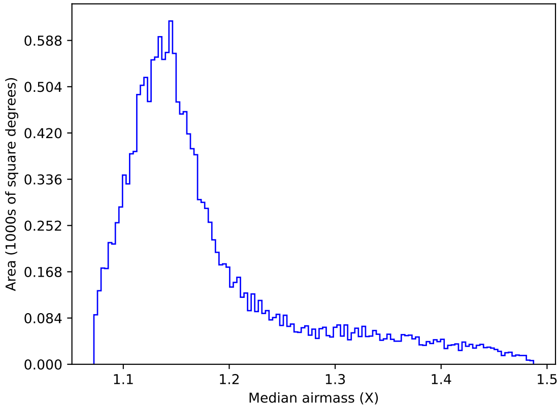
ddf_acor_sf25_lsf40_lsr20_v3.4_10yrs WFD g band: Median airmass
