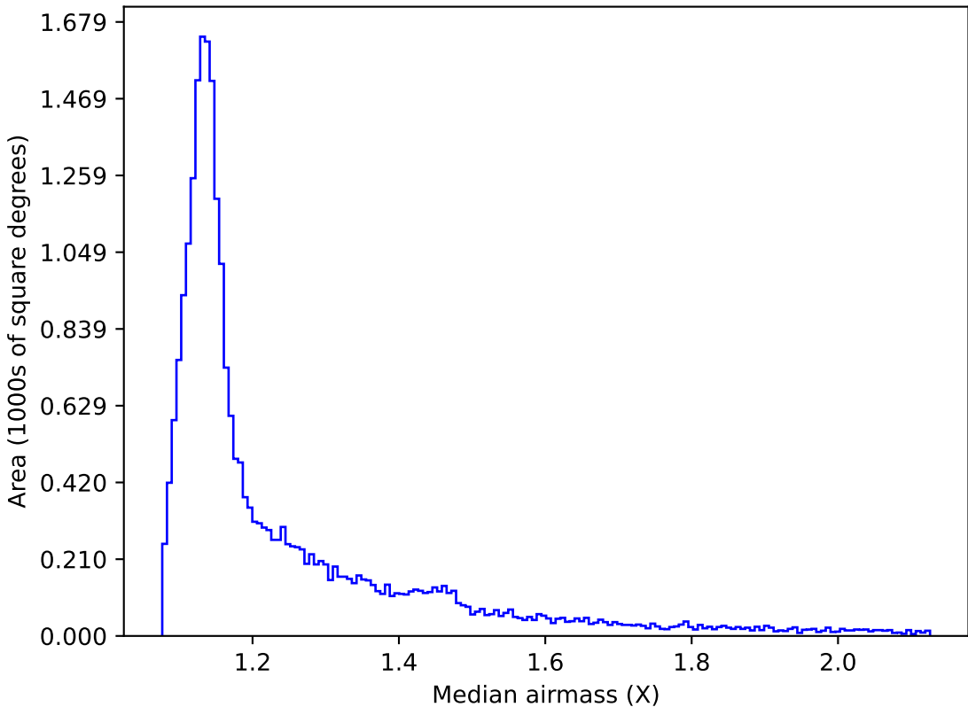
ddf_acor_sf25_lsf40_lsr20_v3.4_10yrs All sky r band: Median airmass
