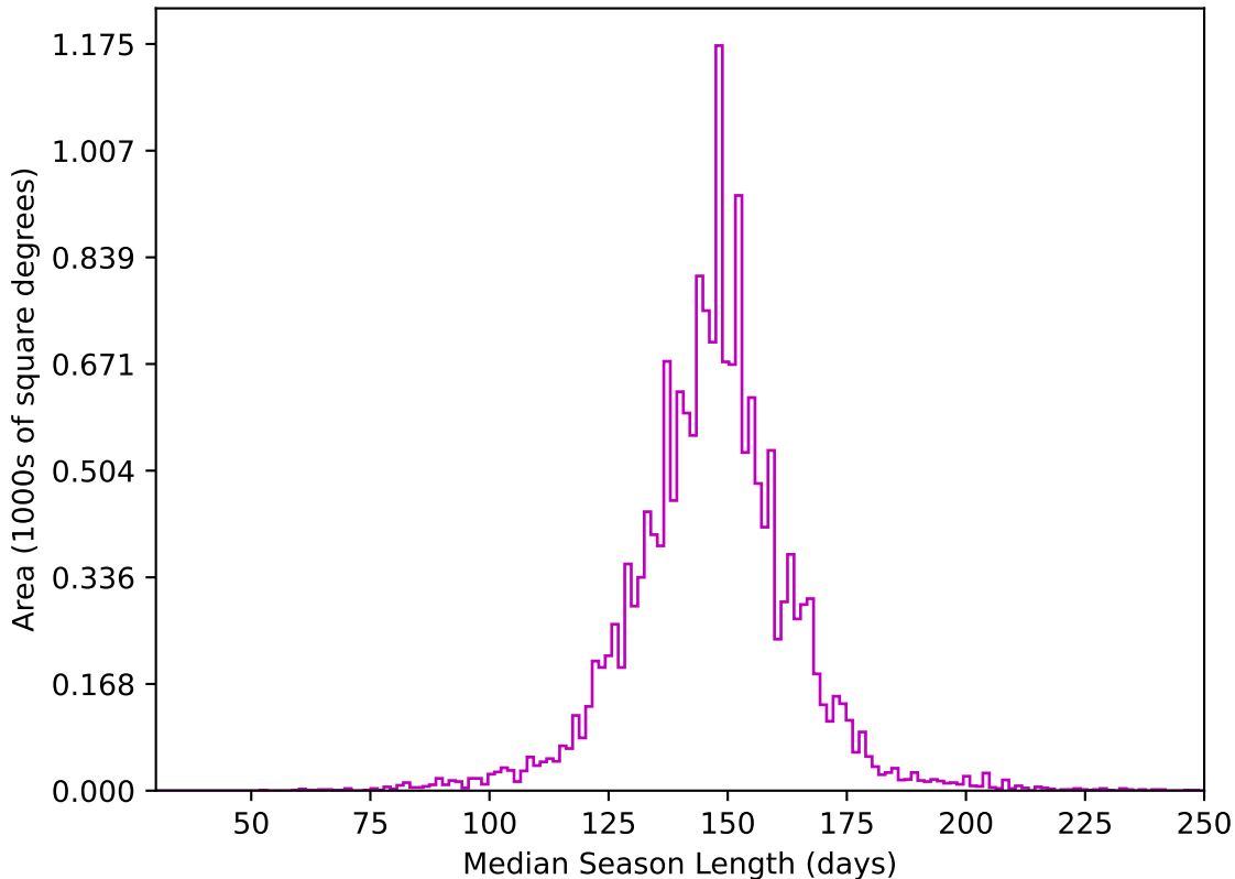
ddf_acor_sf25_lsf40_lsr20_v3.4_10yrs WFD z band: Median Season Length
