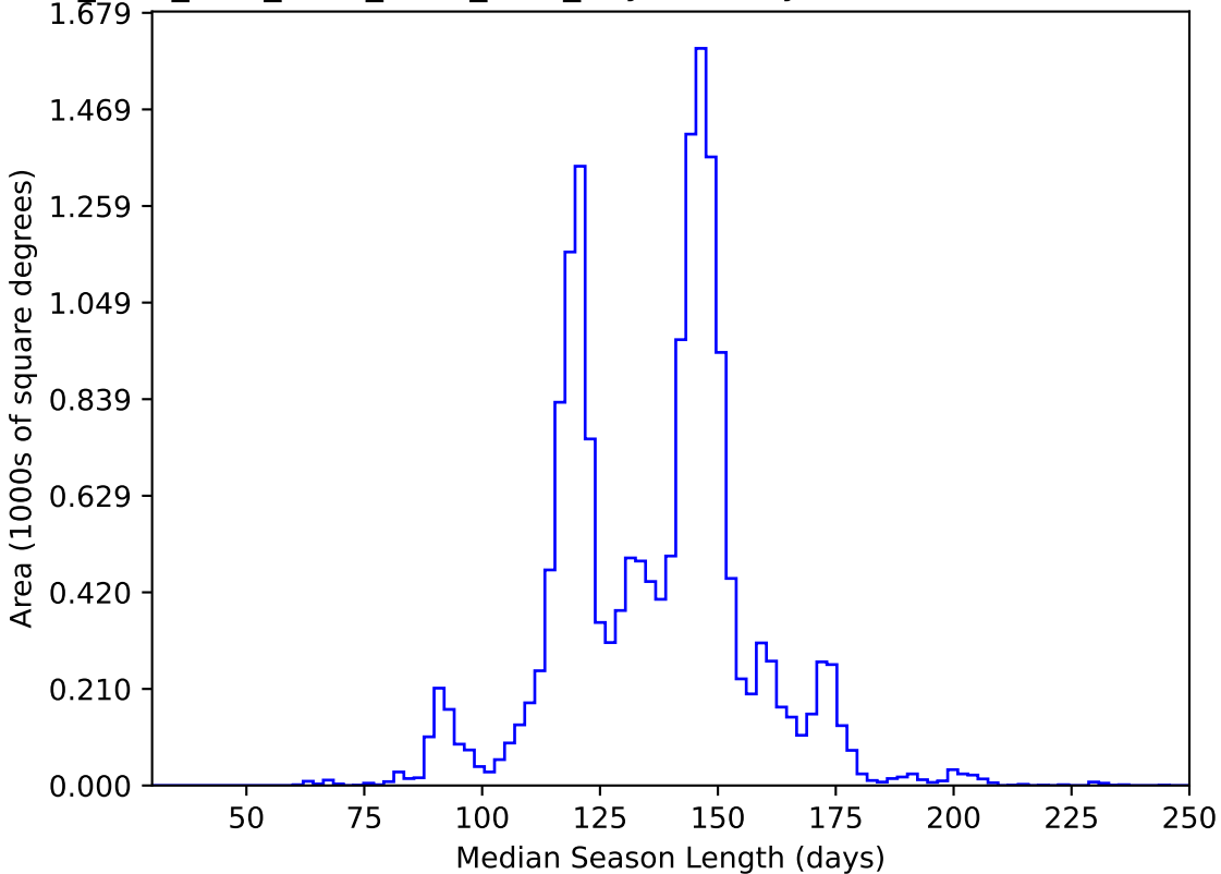
ddf_acor_sf25_lsf40_lsr20_v3.4_10yrs WFD y band: Median Season Length
