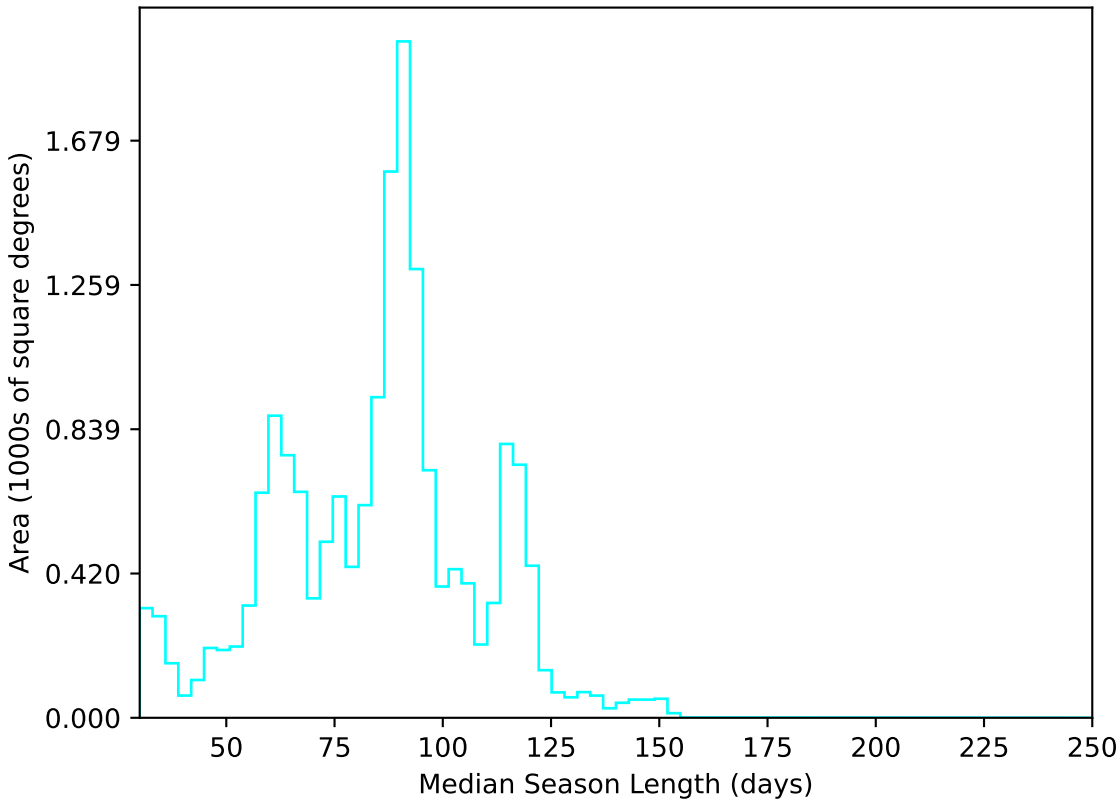
ddf_acor_sf25_lsf40_lsr20_v3.4_10yrs WFD u band: Median Season Length
