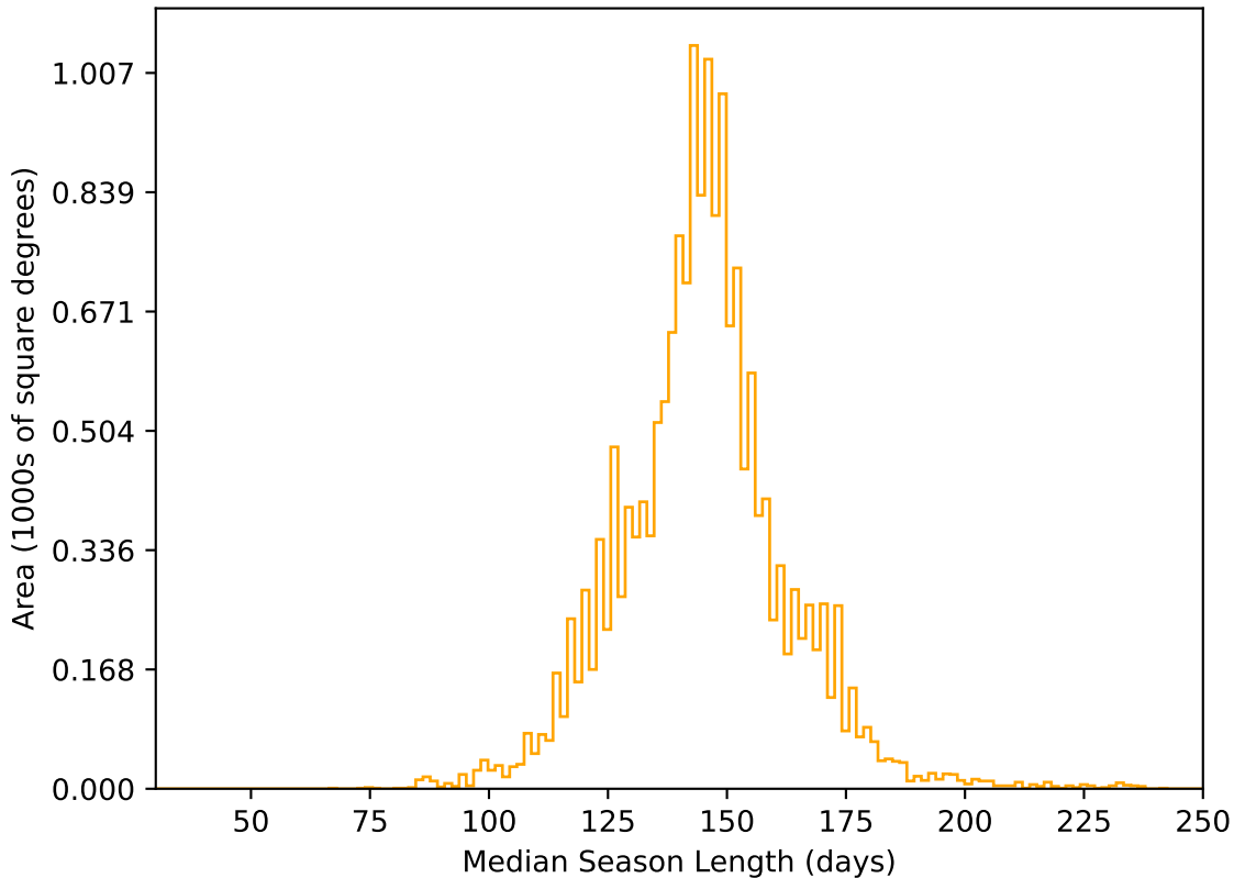
ddf_acor_sf25_lsf40_lsr20_v3.4_10yrs WFD r band: Median Season Length
