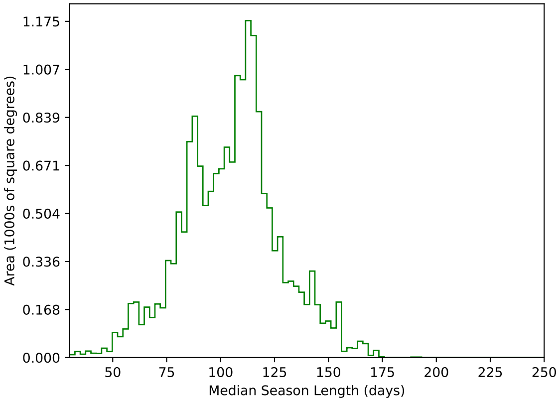
ddf_acor_sf25_lsf40_lsr20_v3.4_10yrs WFD g band: Median Season Length
