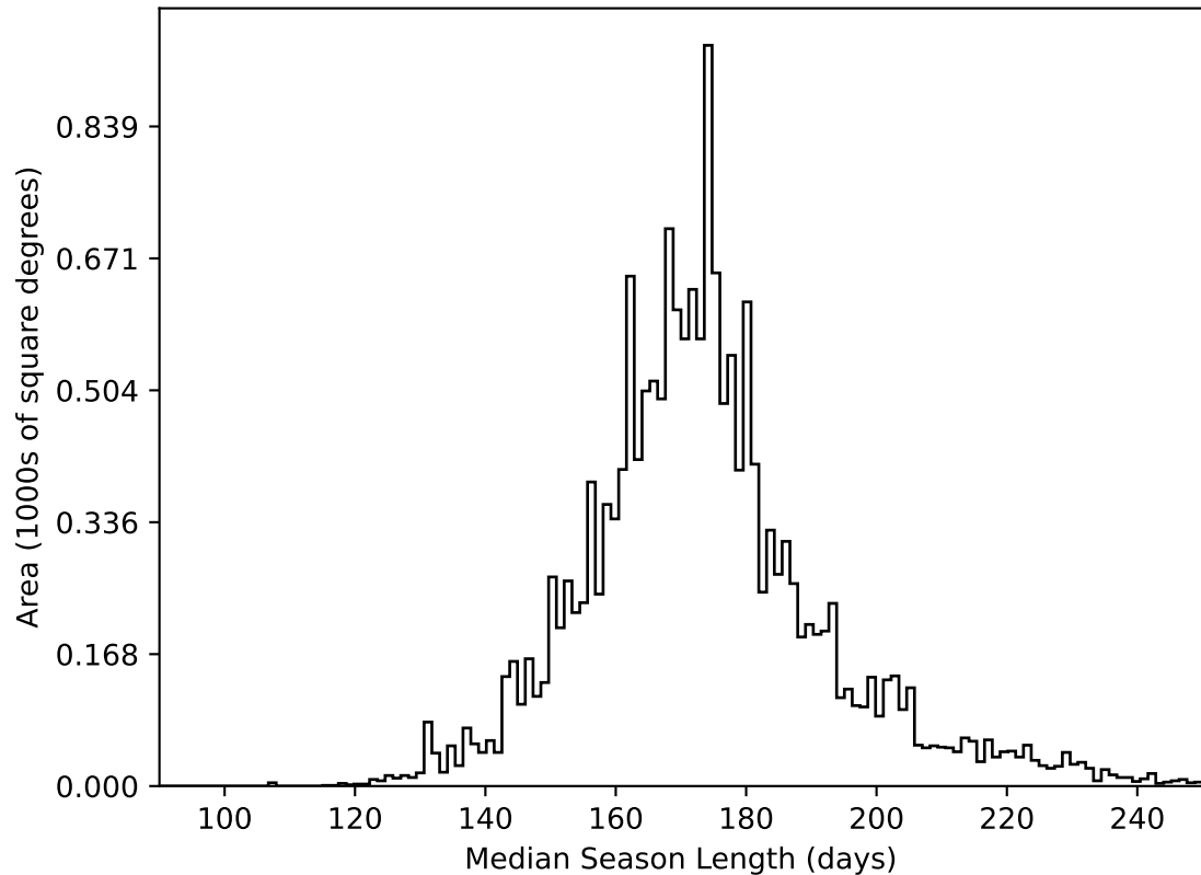
ddf_acor_sf25_lsf40_lsr20_v3.4_10yrs WFD all bands: Median Season Length
