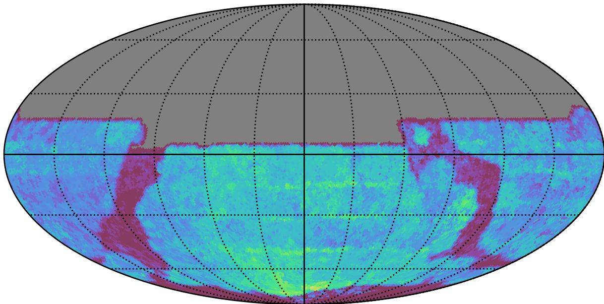
ddf_acor_sf25_lsf40_lsr20_v3.4_10yrs All sky y band: Median Season Length
