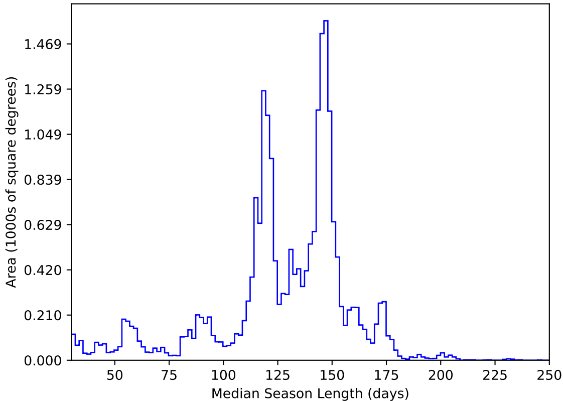
ddf_acor_sf25_lsf40_lsr20_v3.4_10yrs All sky y band: Median Season Length
