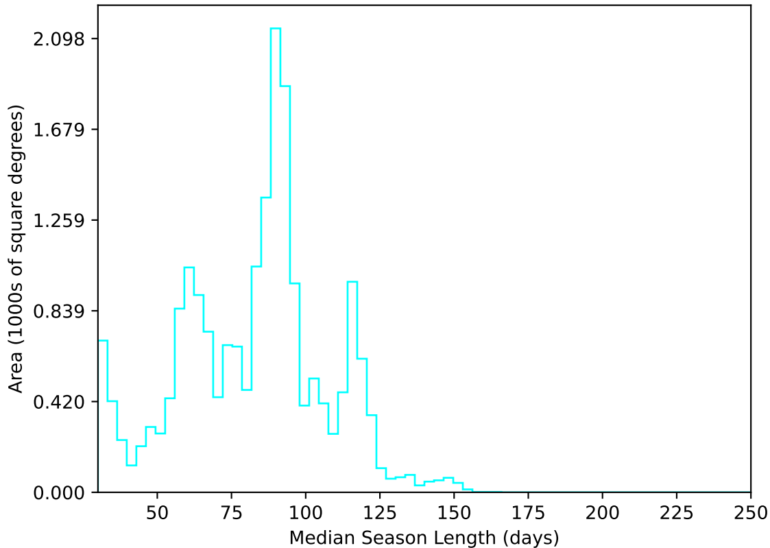
ddf_acor_sf25_lsf40_lsr20_v3.4_10yrs All sky u band: Median Season Length
