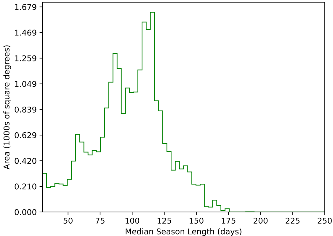
ddf_acor_sf25_lsf40_lsr20_v3.4_10yrs All sky g band: Median Season Length
