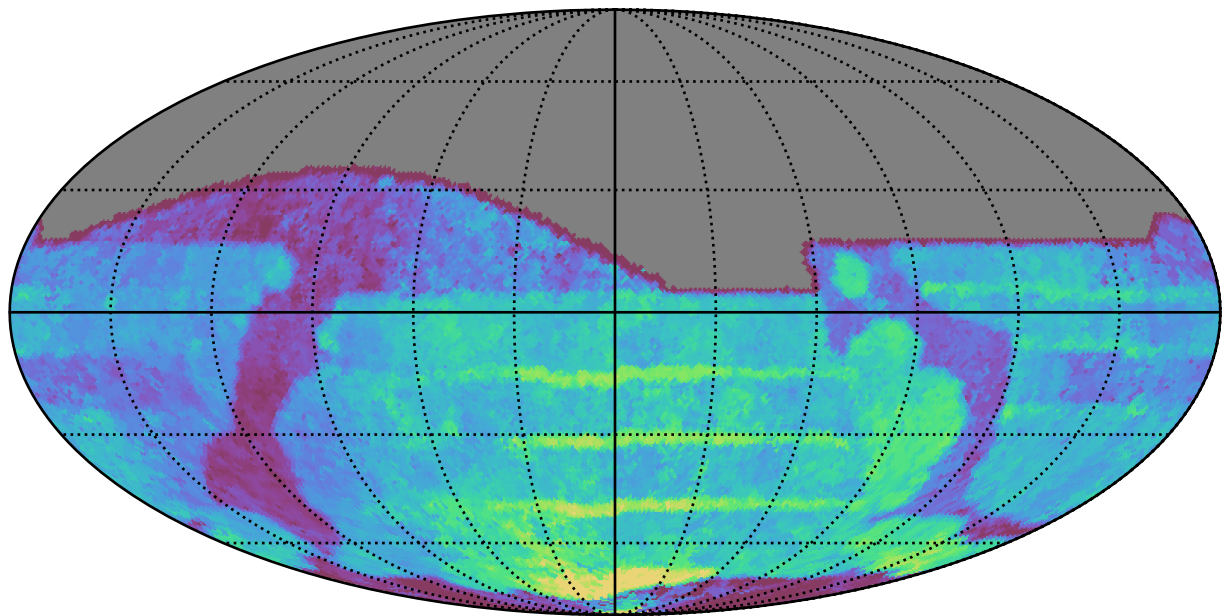
ddf_acor_sf25_lsf40_lsr20_v3.4_10yrs All sky all bands: Median Season Length
