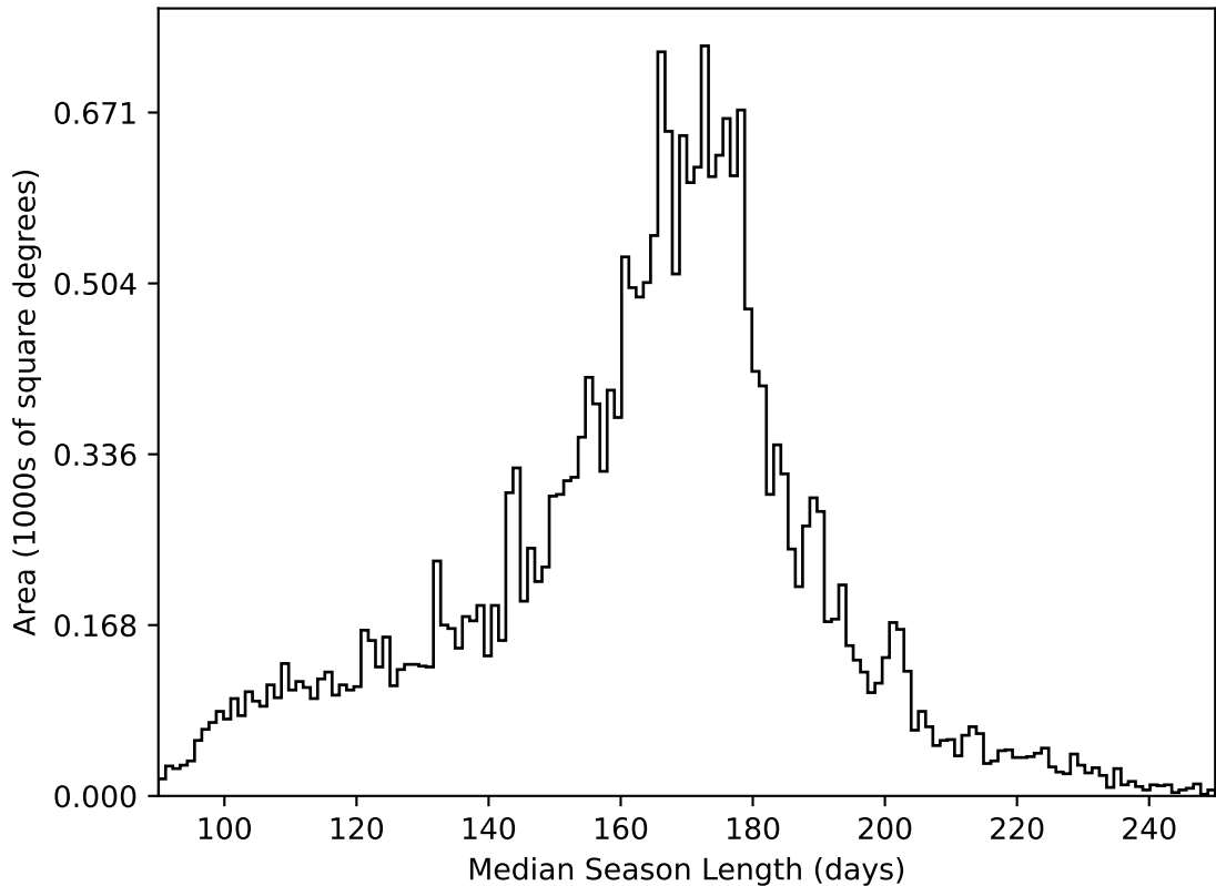
ddf_acor_sf25_lsf40_lsr20_v3.4_10yrs All sky all bands: Median Season Length
