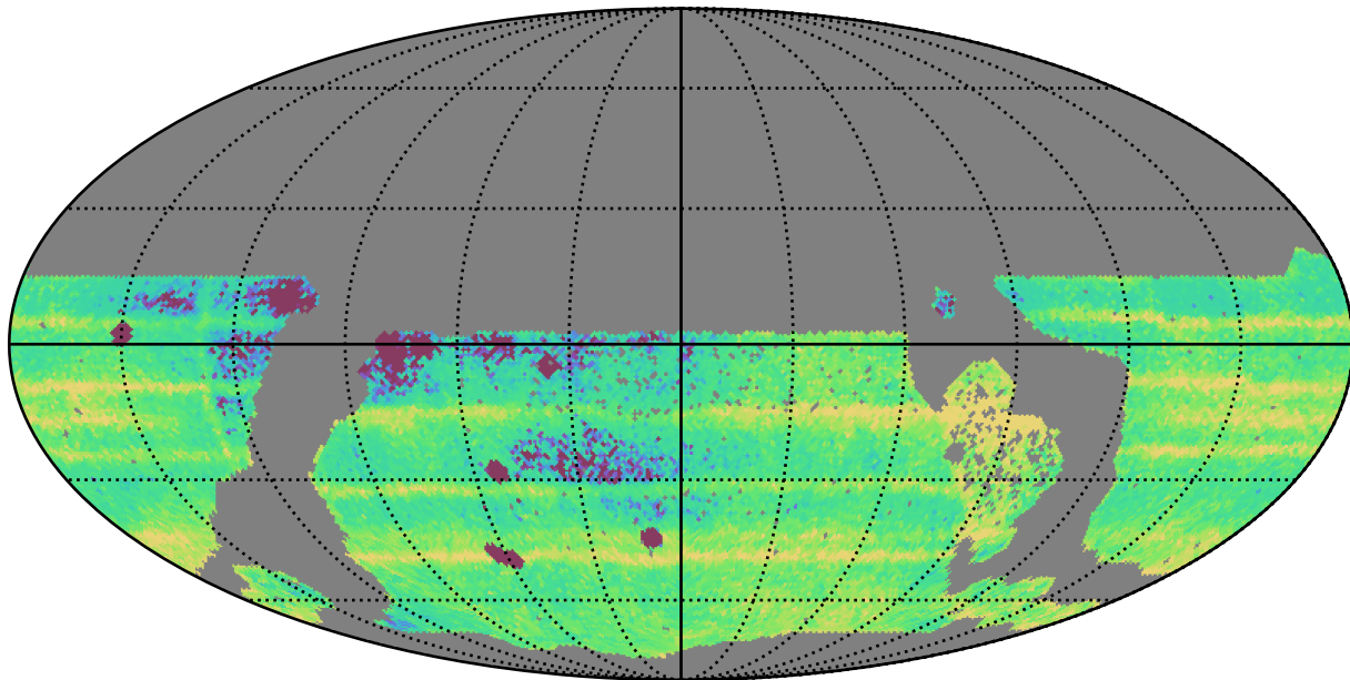
ddf_acor_sf25_lsf40_lsr20_v3.4_10yrs WFD: Median Intra-Night Gap
