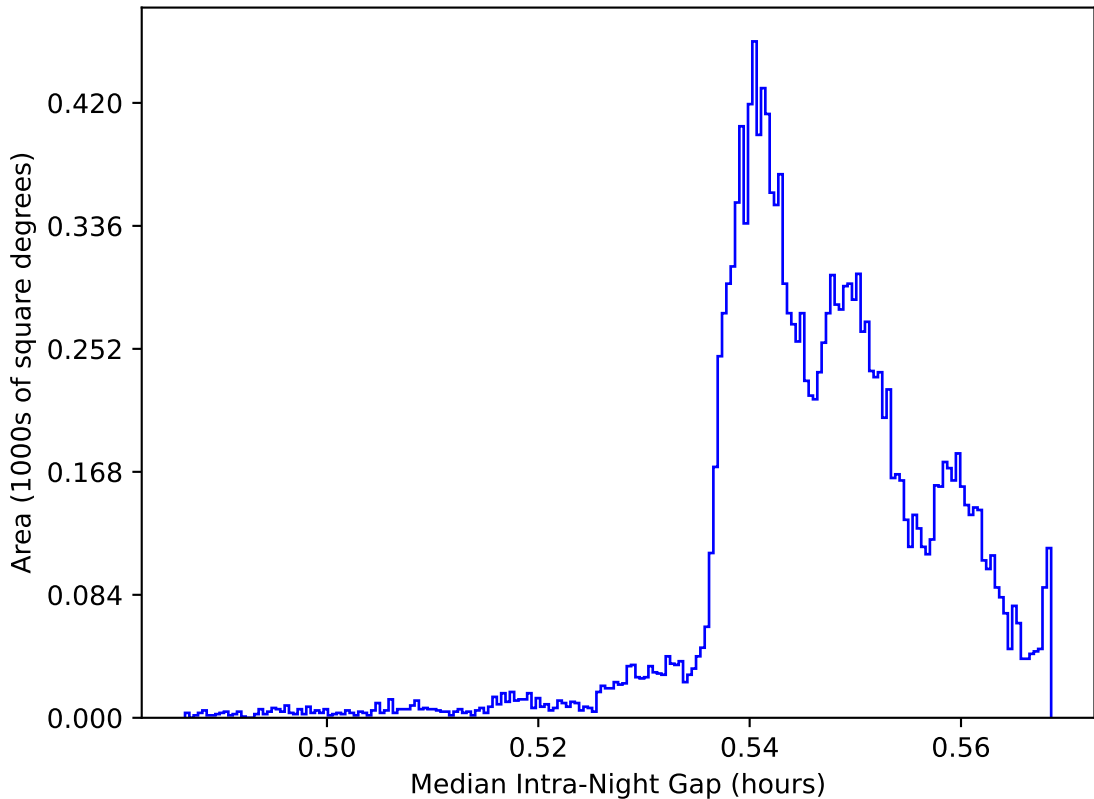
ddf_acor_sf25_ls40_lsr20_v3.4_10yrs WFD: Median Intra-Night Gap
