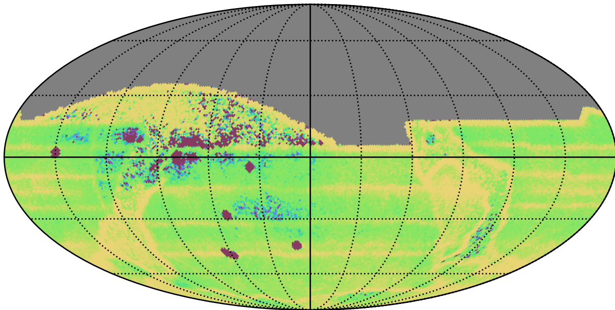
ddf_acor_sf25_lsf40_lsr20_v3.4_10yrs All sky: Median Intra-Night Gap
