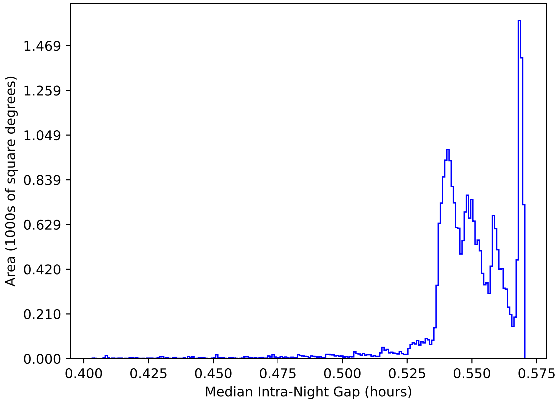
ddf_acor_sf25_lsf40_lsr20_v3.4_10yrs All sky: Median Intra-Night Gap
