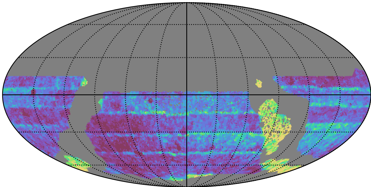
ddf_acor_sf25_lsf40_lsr20_v3.4_10yrs WFD z band: Median Inter-Night Gap
