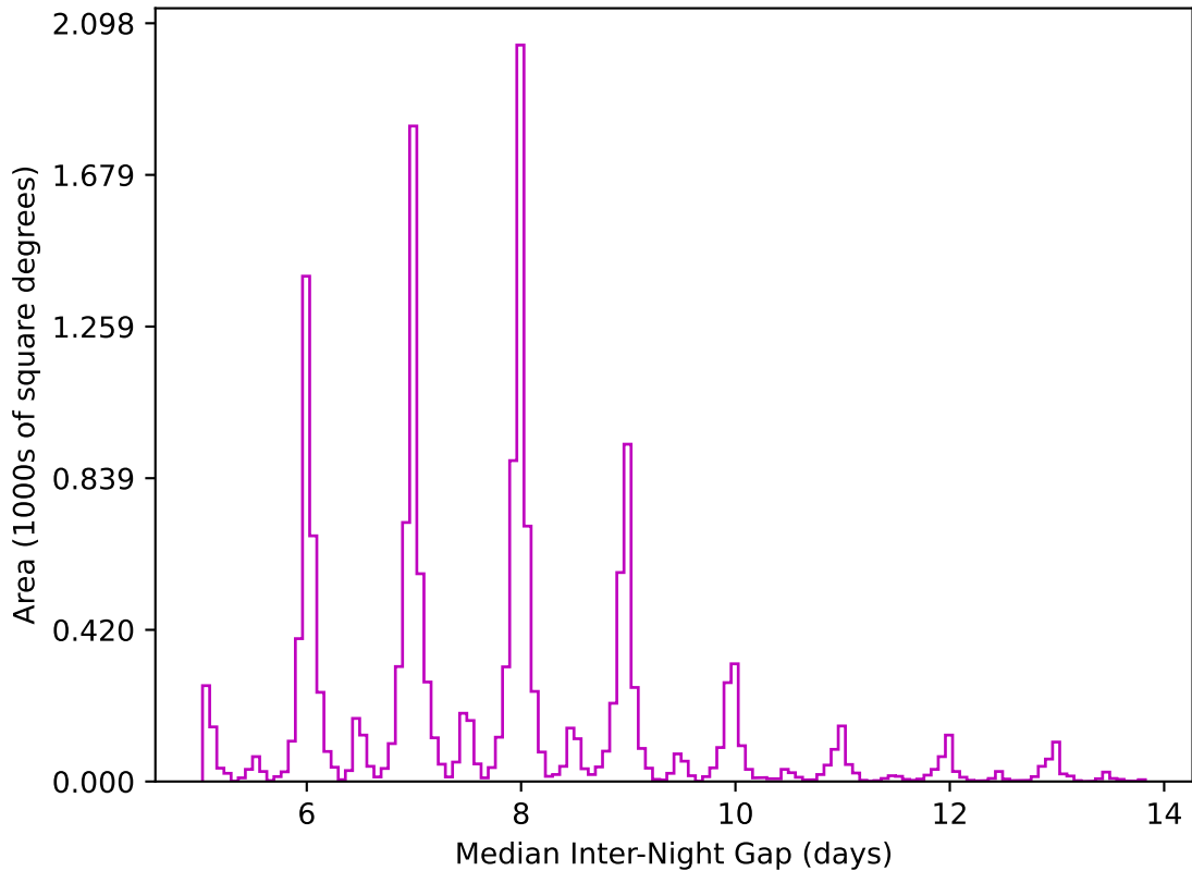
ddf_acor_sf25_lsf40_lsr20_v3.4_10yrs WFD z band: Median Inter-Night Gap
