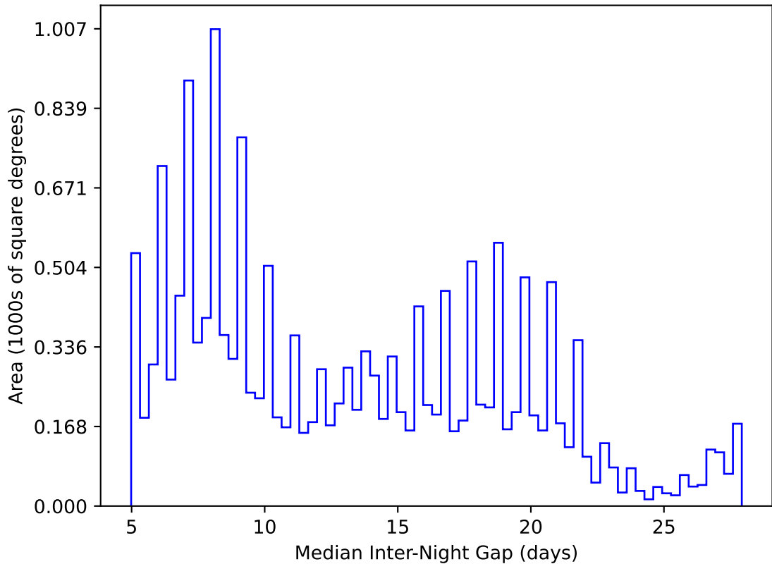
ddf_acor_sf25_lsf40_lsr20_v3.4_10yrs WFD y band: Median Inter-Night Gap
