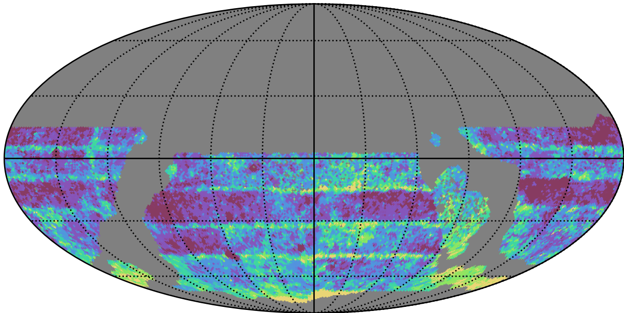
ddf_acor_sf25_lsf40_lsr20_v3.4_10yrs WFD r band: Median Inter-Night Gap
