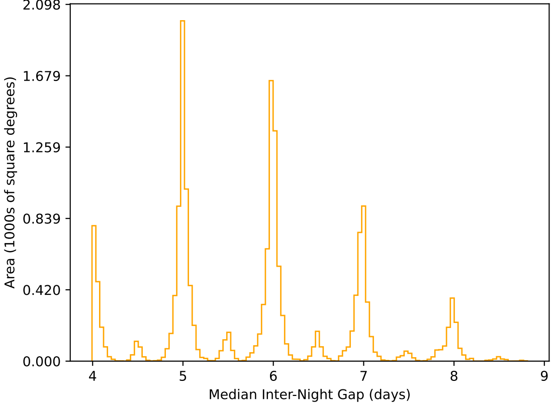
ddf_acor_sf25_ls40_lsr20_v3.4_10yrs WFD r band: Median Inter-Night Gap
