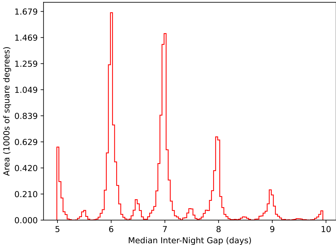
ddf_acor_sf25_lsf40_lsr20_v3.4_10yrs WFD i band: Median Inter-Night Gap
