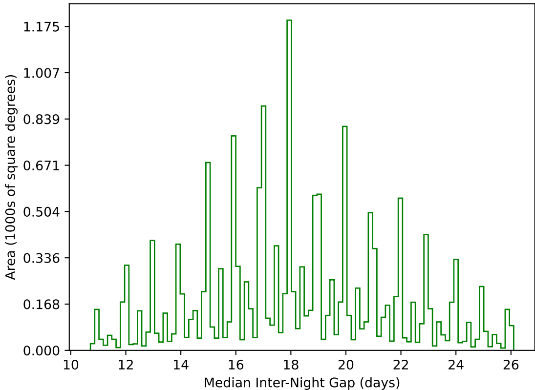
ddf_acor_sf25_lsf40_lsr20_v3.4_10yrs WFD g band: Median Inter-Night Gap
