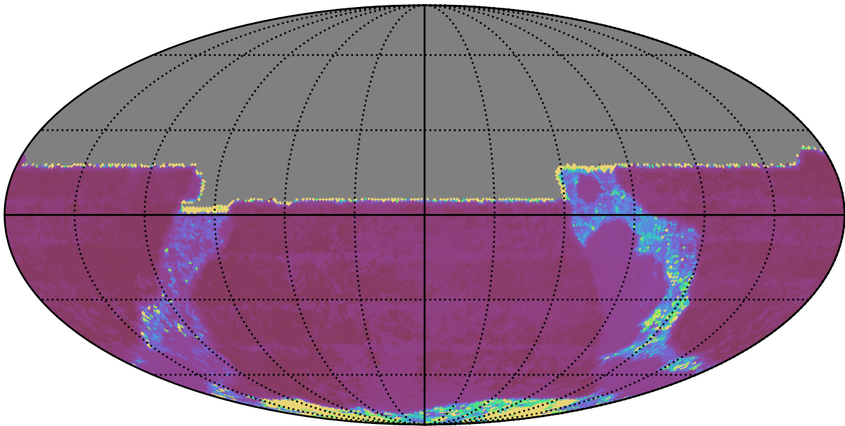
ddf_acor_sf25_lsf40_lsr20_v3.4_10yrs All sky y band: Median Inter-Night Gap
