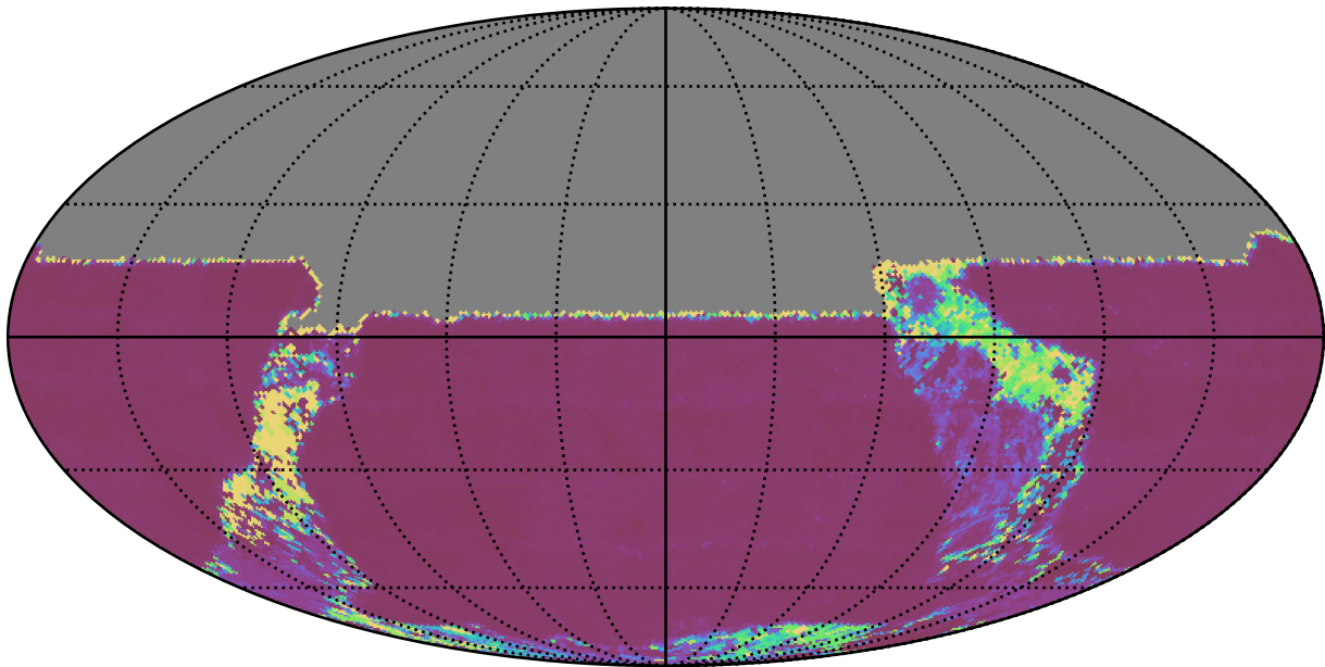
ddf_acor_sf25_lsf40_lsr20_v3.4_10yrs All sky u band: Median Inter-Night Gap
