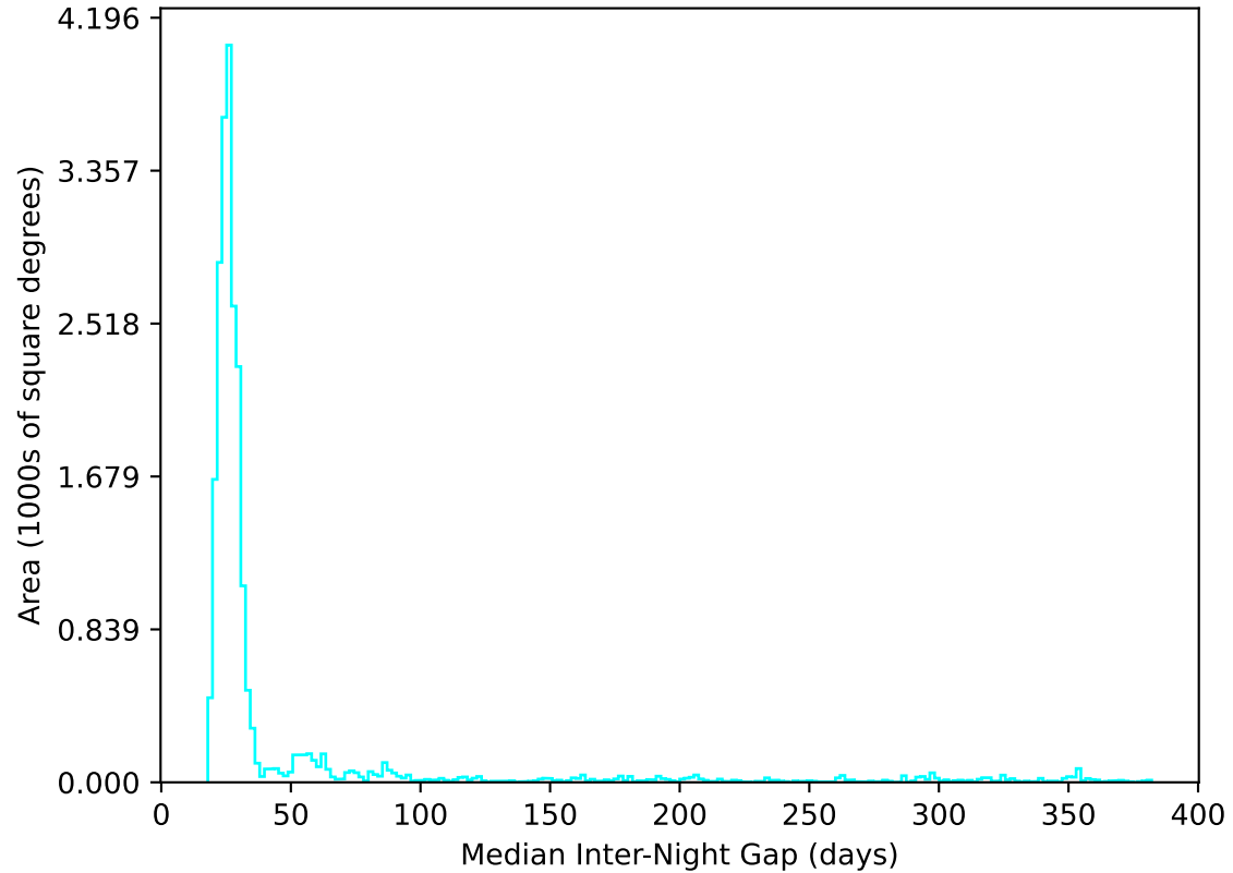
ddf_acor_sf25_lsf40_lsr20_v3.4_10yrs All sky u band: Median Inter-Night Gap
