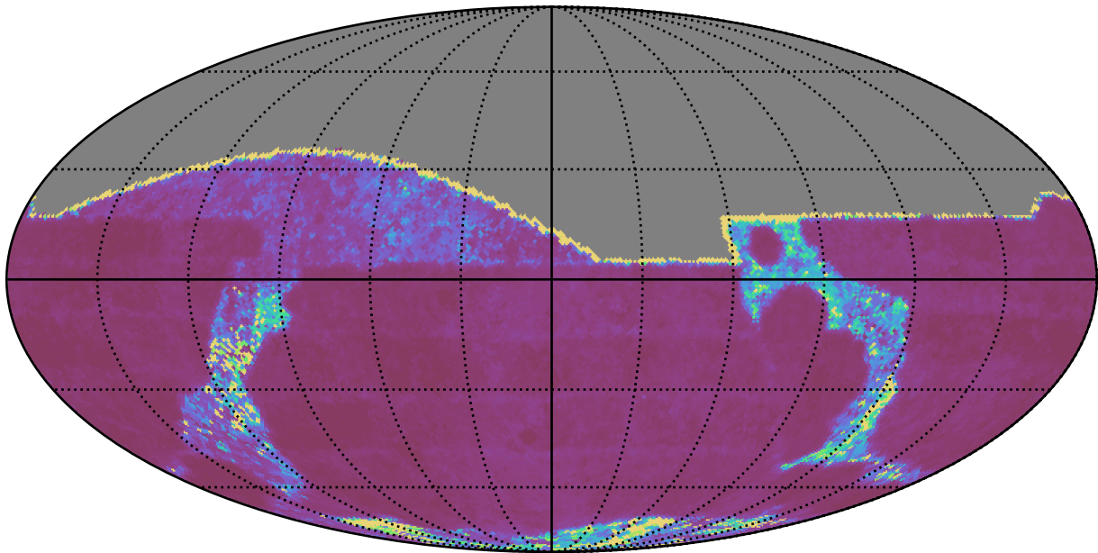
ddf_acor_sf25_lsf40_lsr20_v3.4_10yrs All sky g band: Median Inter-Night Gap
